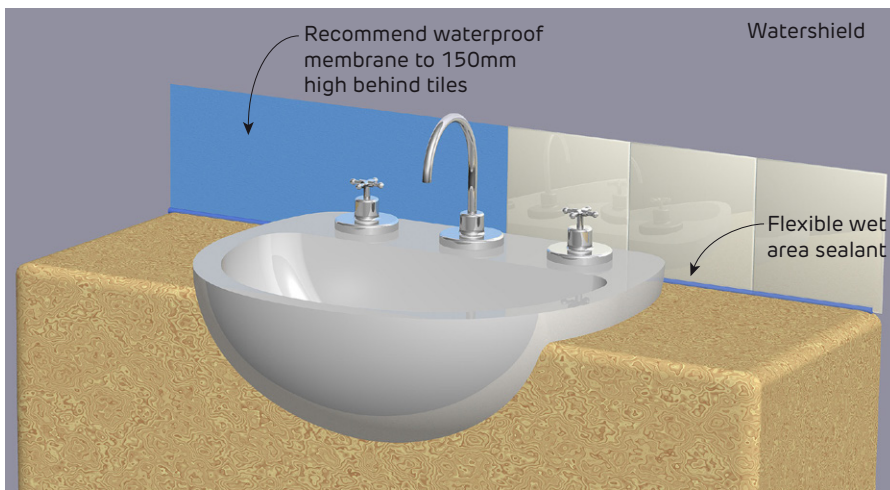
FIGURE 44 Basin
