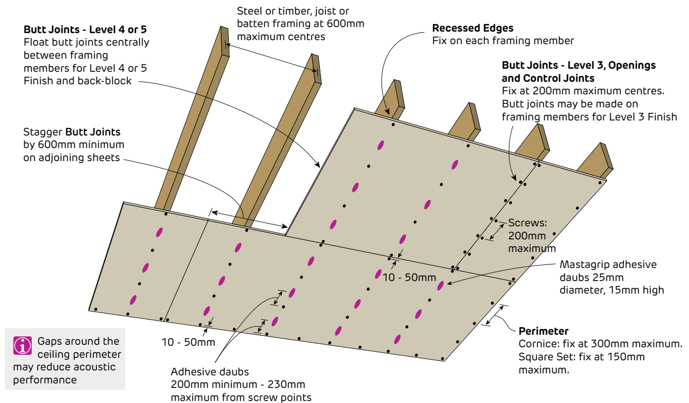
FIGURE 20 Internal Garage Ceiling - 1 Layer One Third Fastener and Adhesive Method
