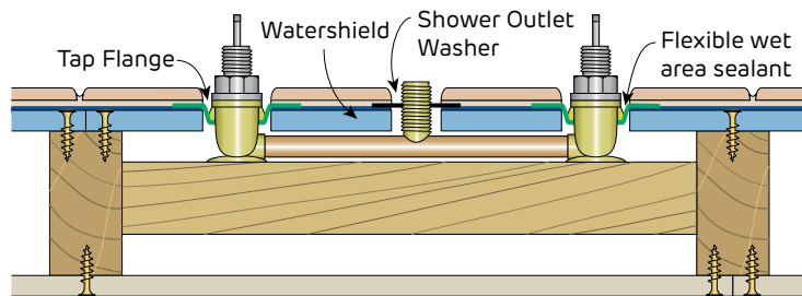
FIGURE 58 Alternative Plumbing Penetrations Proprietary tap flange and shower outlet washer Plan
