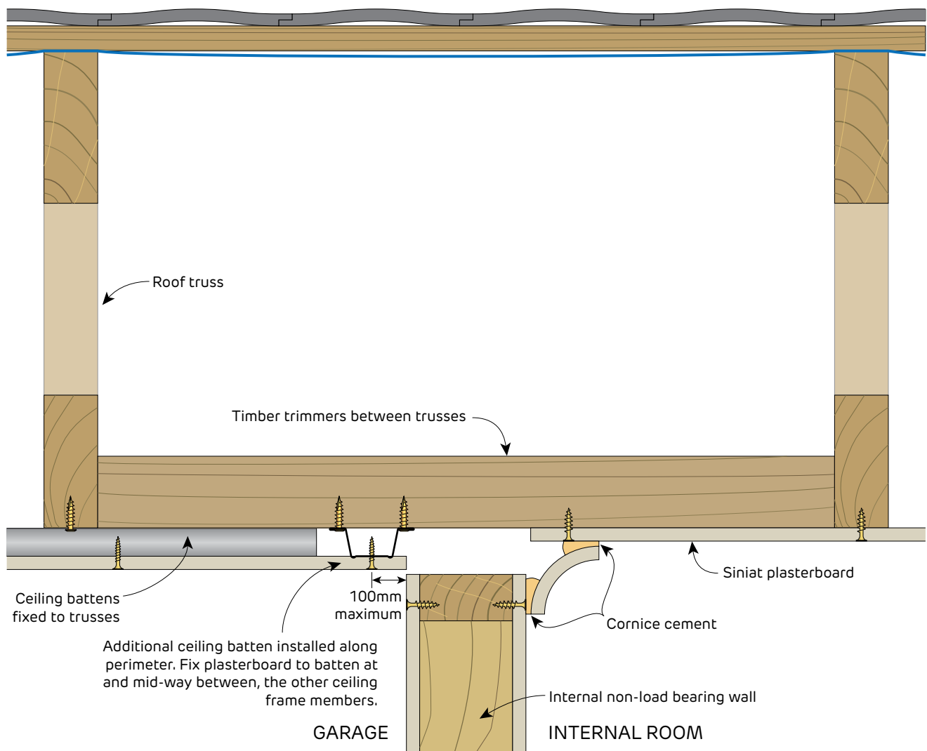
FIGURE 19 Plasterboard Ceiling Perimeter Detail Cornice Only
