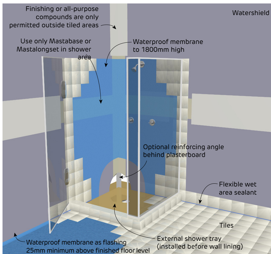
FIGURE 47 External tray for enclosed shower on timber flooring
