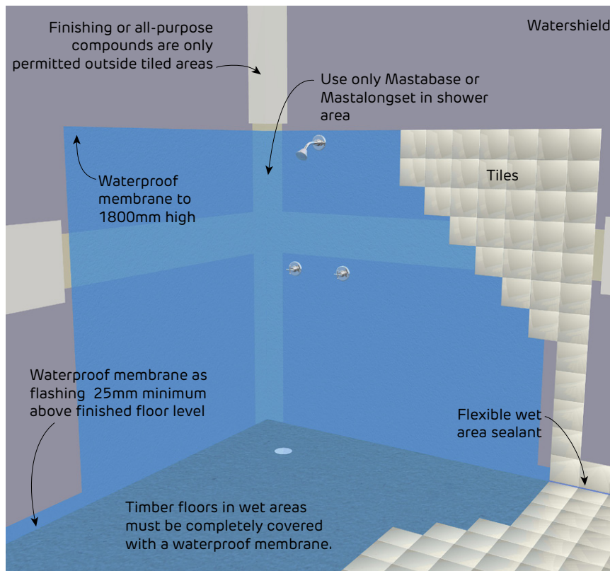
FIGURE 46 Internal in situ tray on timber flooring
