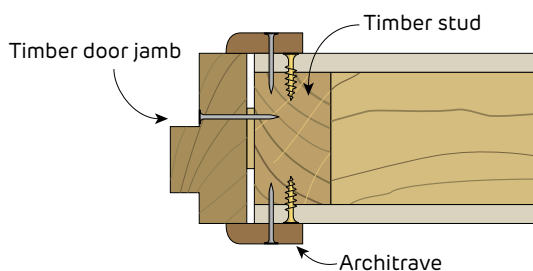
FIGURE 37 Timber Door jamb Plan
