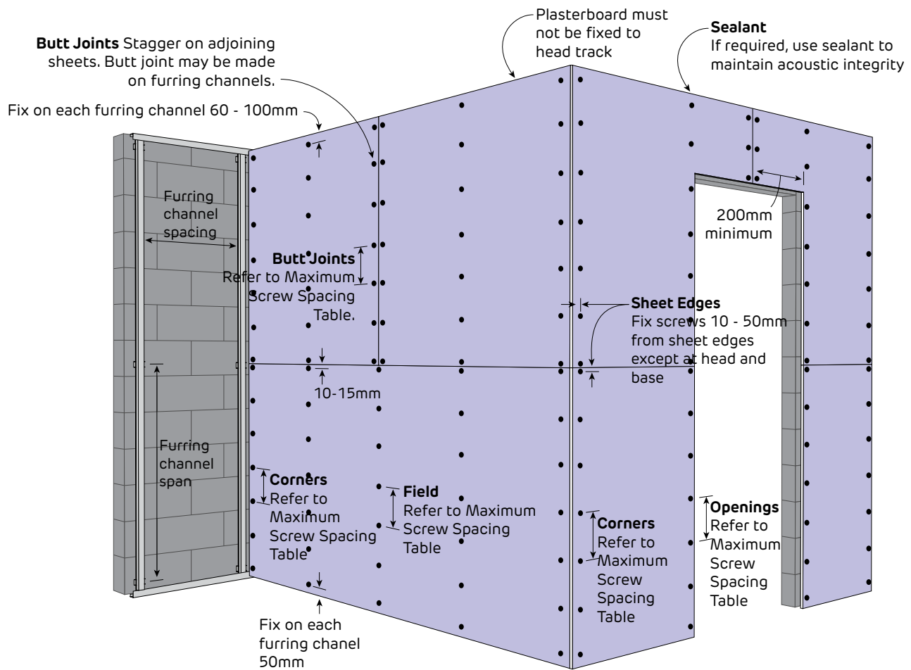
FIGURE 50 Watershield in Tiled Areas - 1 Layer Horizontal Screw Only Method over furring channels
