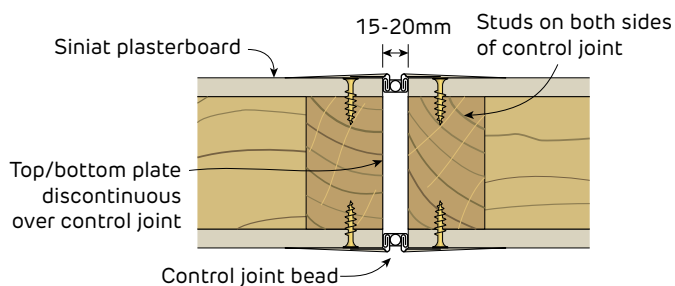
FIGURE 34 Wall Control Joint Plan
