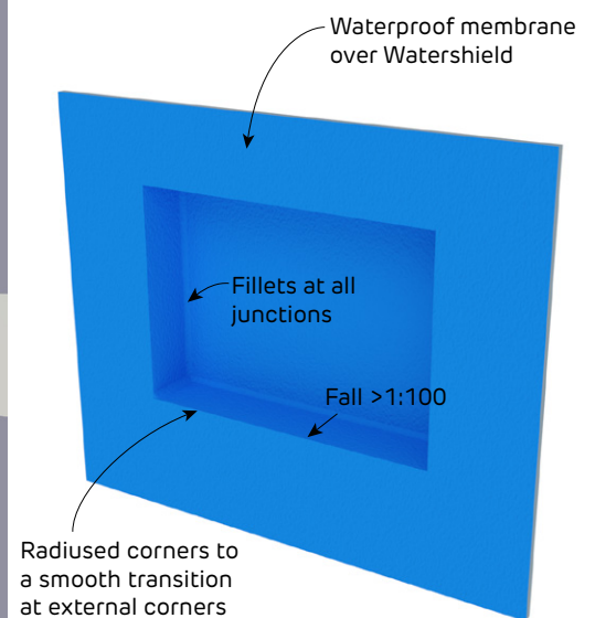
FIGURE 48 Niche
