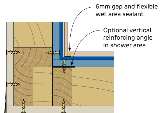
FIGURE 54 Shower Corner Plan
