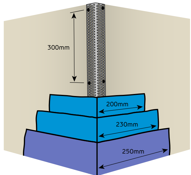
FIGURE 71 External Corner
