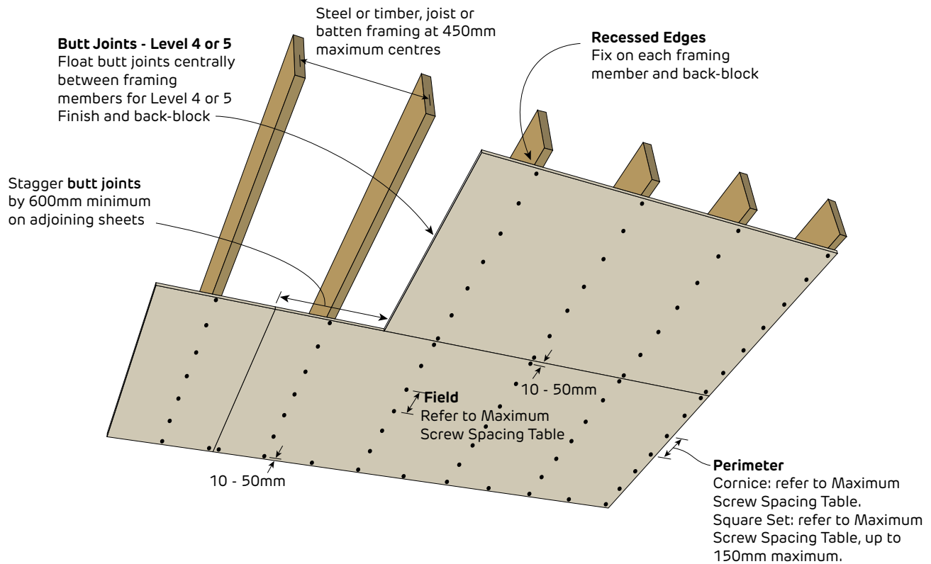
FIGURE 21 External Ceiling - 1 Layer Screw Only Method
