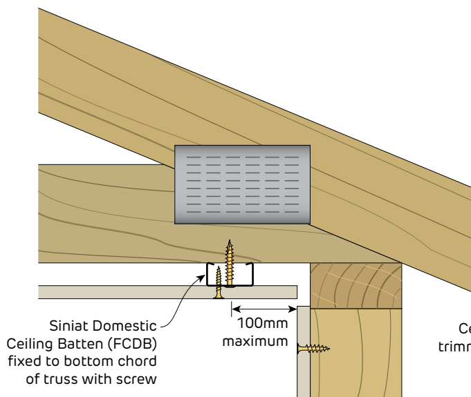
FIGURE 11 Direct Fix Ceiling to Roof Truss 16mm Domestic Batten fixed directly to trusses Section
