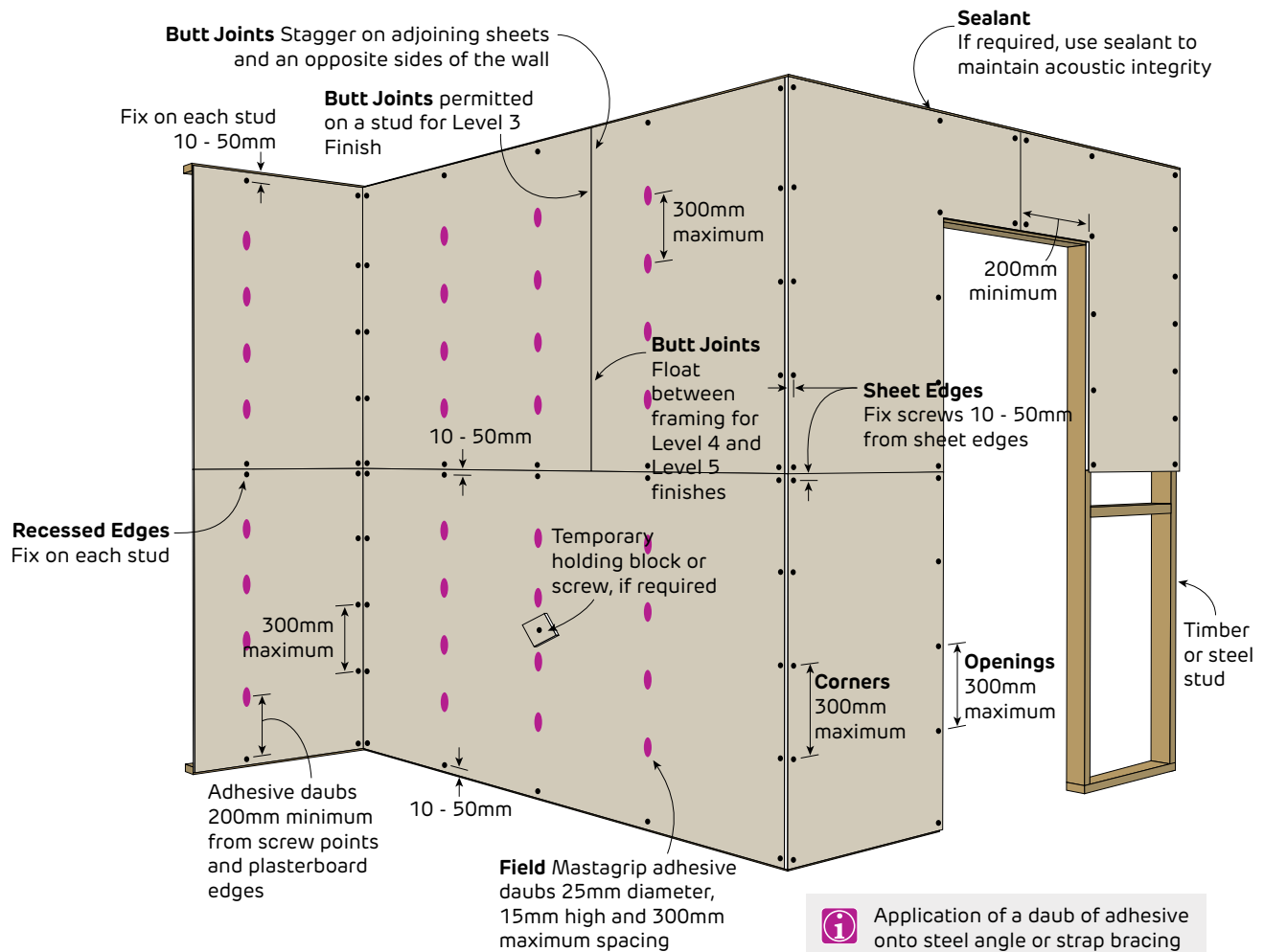
FIGURE 28 Internal Wall - 1 Layer Horizontal Fastener and Adhesive Method
