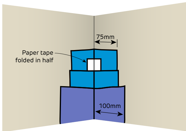
FIGURE 70 Internal Corner
