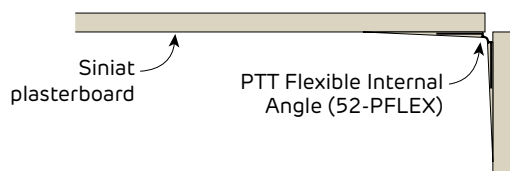
FIGURE 18 Finishing Detail - Flexible Square Set Section
