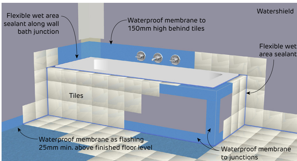
FIGURE 45 Bath (without shower) installation on timber flooring
