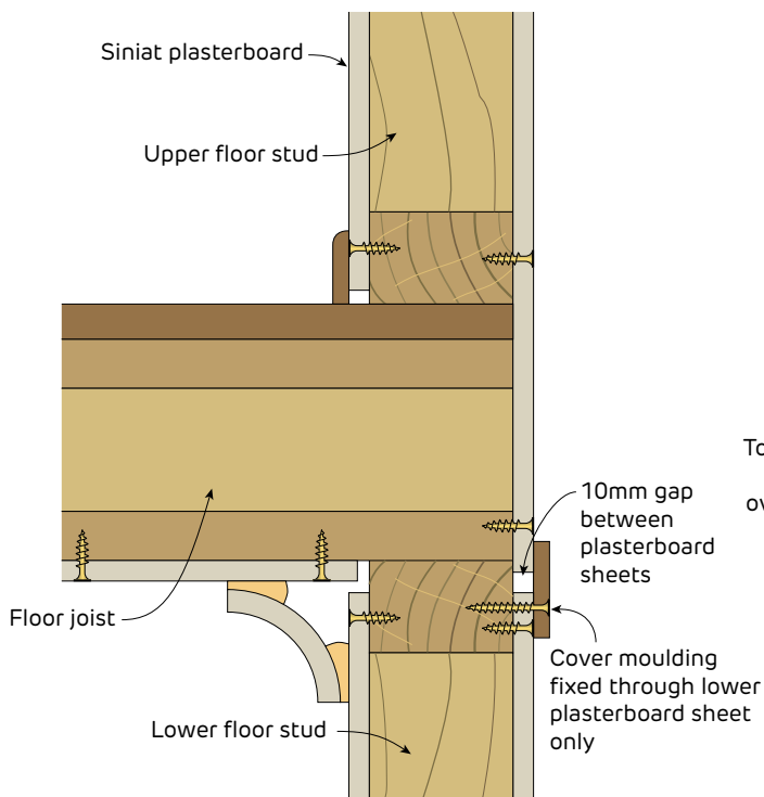
FIGURE 35 Horizontal Control Joint at Mid-floor Section
