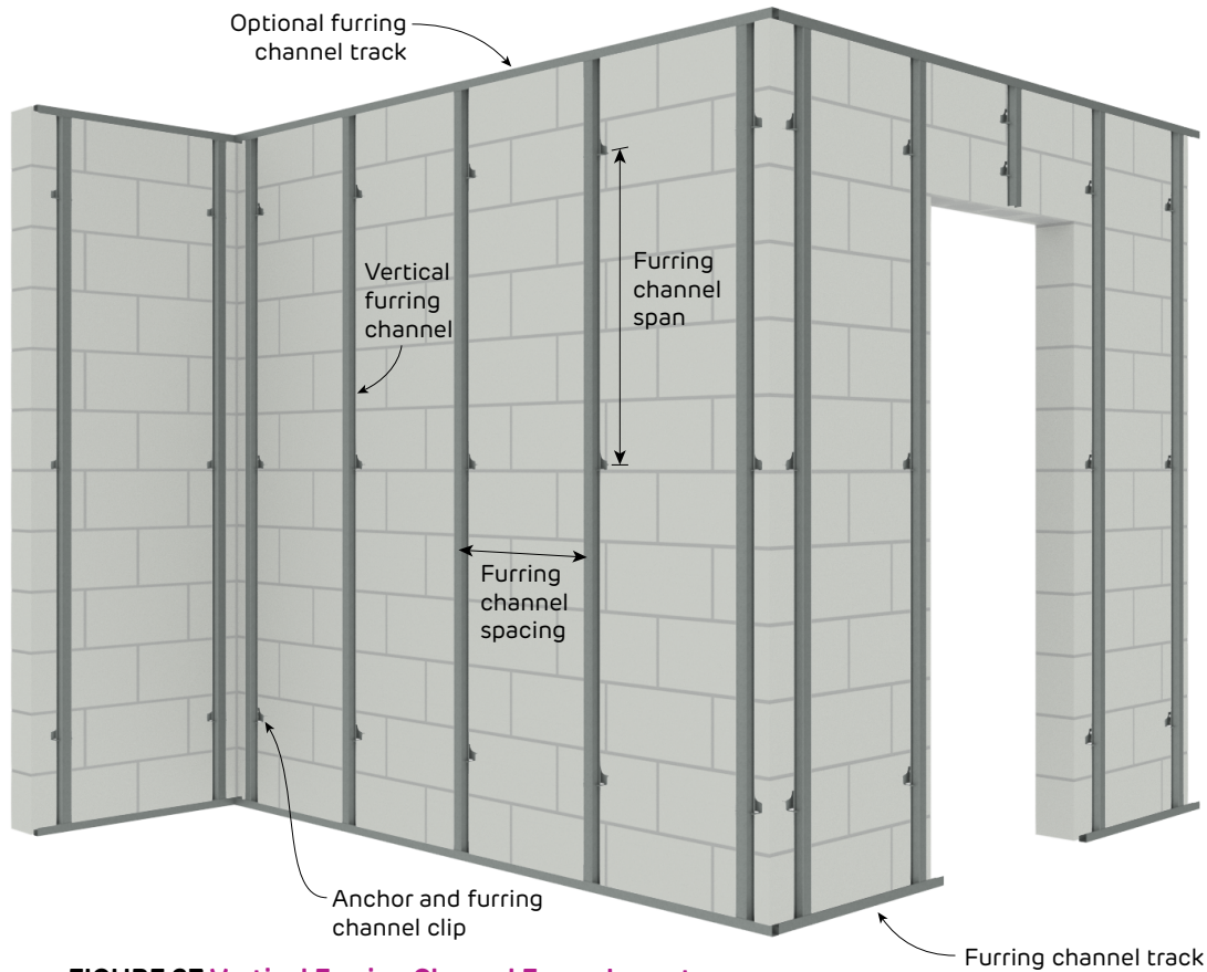
FIGURE 27 Vertical Furring Channel Frame Layout
