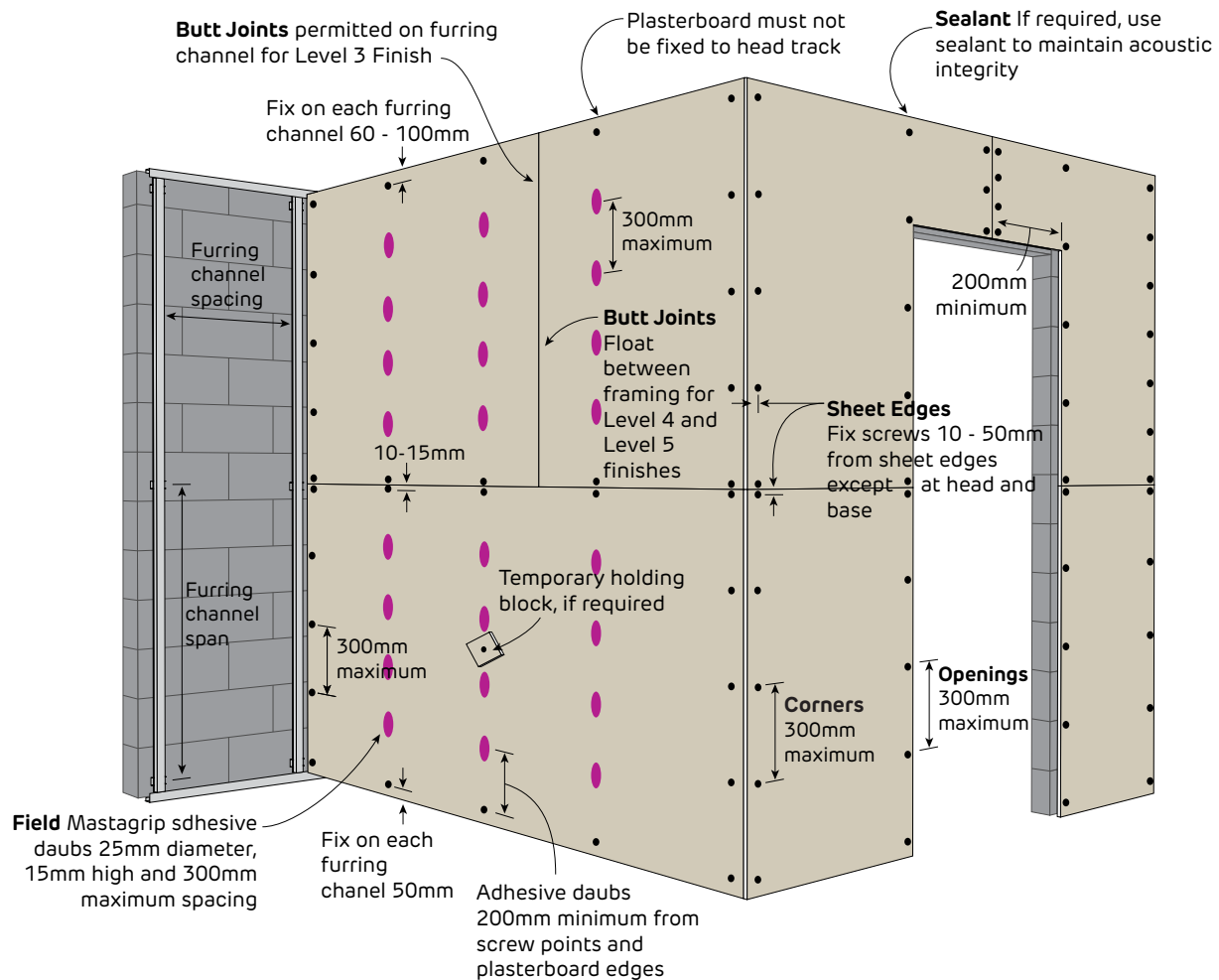
FIGURE 32 Internal Wall - 1 Layer Horizontal Screw and Adhesive Method over furring channels
