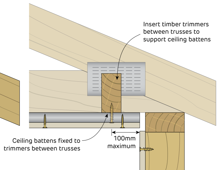
FIGURE 12 Direct Fix Ceiling to Roof Truss 16mm Domestic Batten fixed directly to trusses Section
