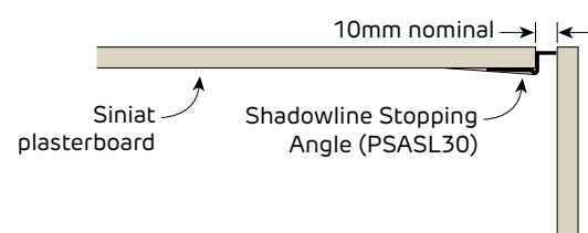
FIGURE 17 Finishing Detail - Shadowline Section
