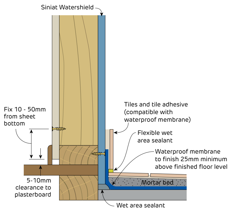
FIGURE 55 Wall Base in General Wet Area Outside shower - Class 3 membrane shown Section
