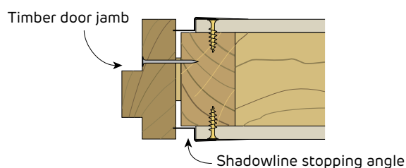
FIGURE 39 Timber Door jamb With Shadowline Stopping Angle - Plan
