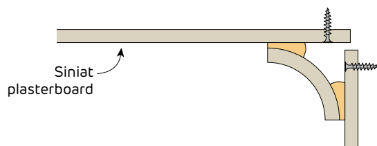
FIGURE 16 Finishing Detail - Cornice Section
