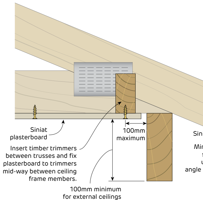
FIGURE 22 Plasterboard Ceiling Fixed to Roof Truss With perimeter timber trimmers between trusses Section
