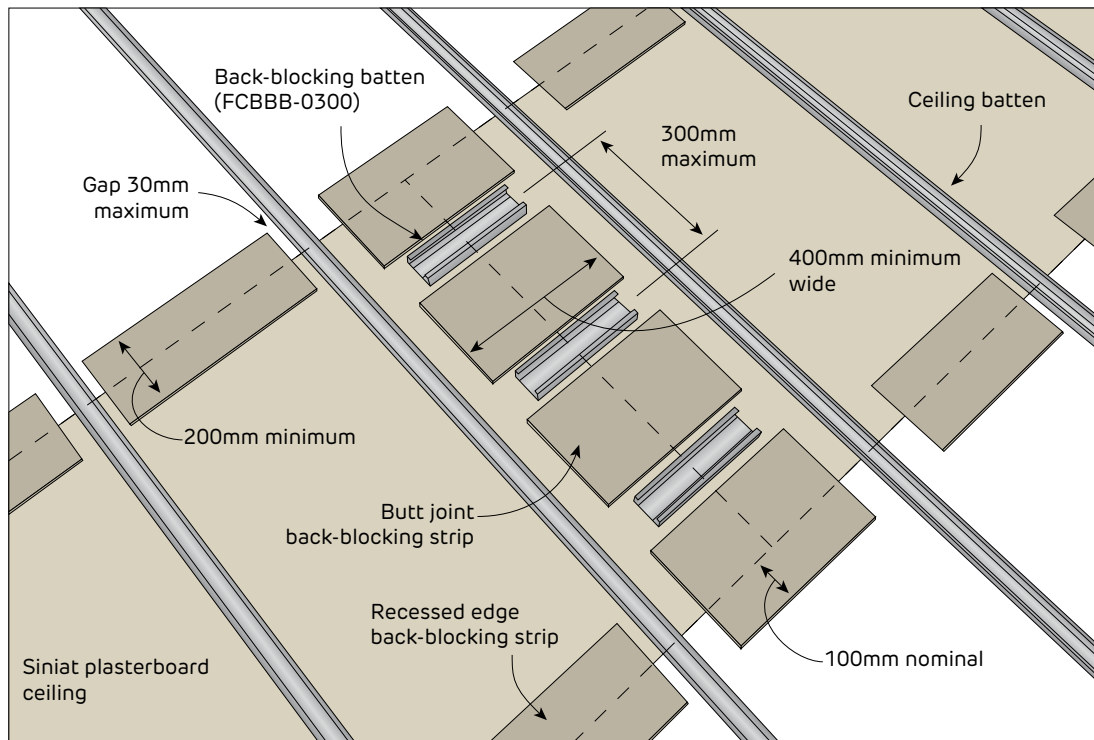
FIGURE 61 Placement of Back-Blocking Batten and Back-Blocking Strips for Recessed and Butt Joints
