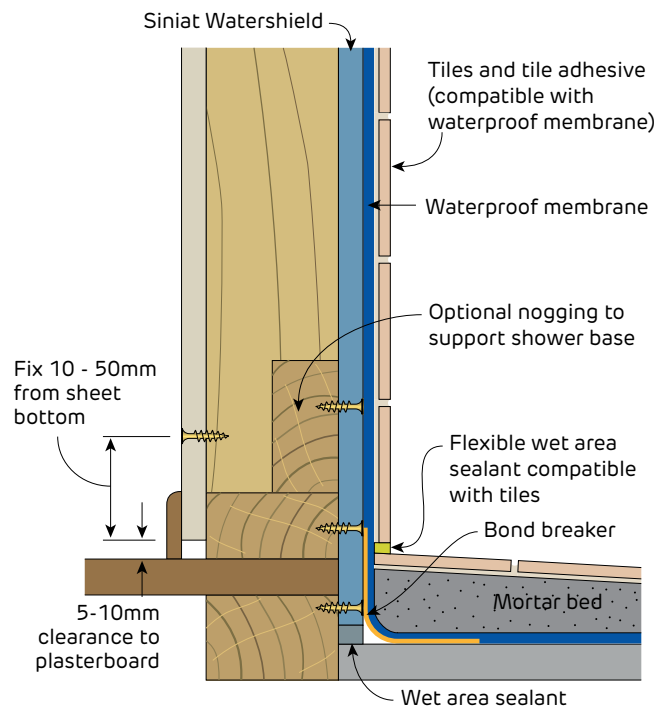
FIGURE 52 Shower Base Shower with dropdown Class 2 membrane shown - Section
