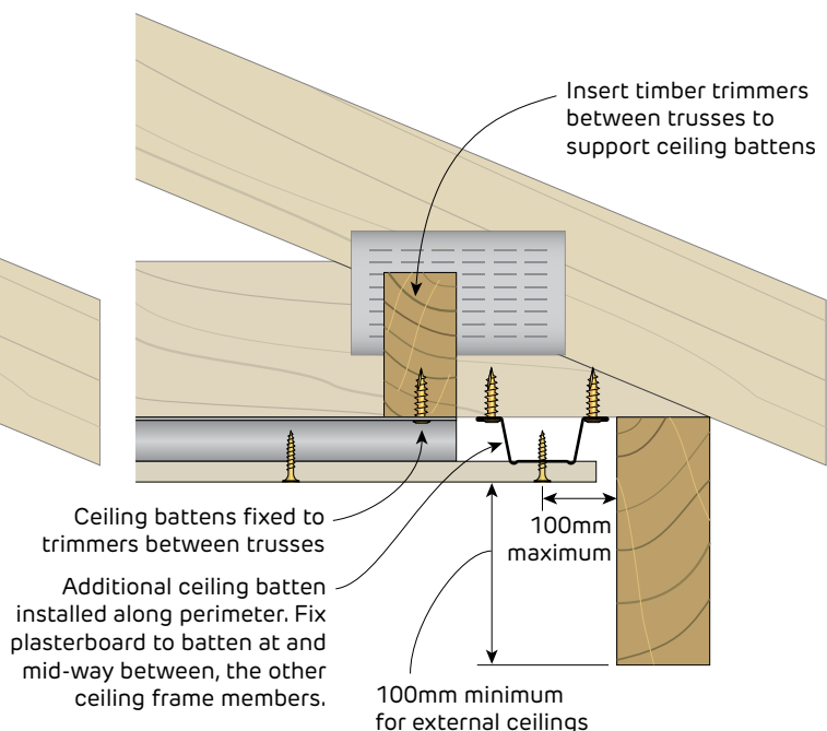
FIGURE 25 Plasterboard Ceiling Fixed to Battens Ceiling battens installed parallel to trusses Section
