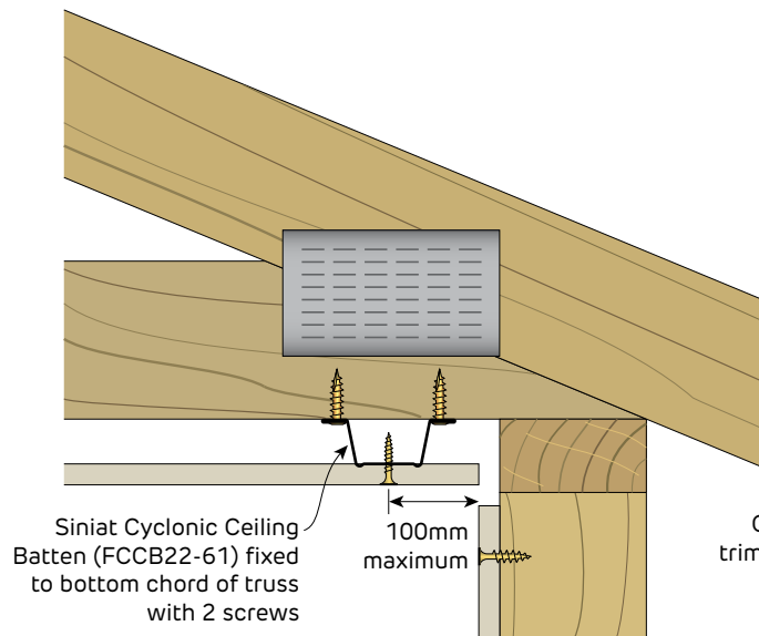
FIGURE 14 Direct Fix Ceiling to Roof Truss 22mm Cyclonic Batten perpendicular to trusses Section
