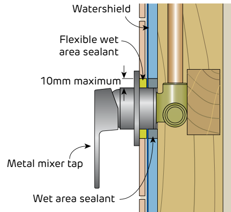
FIGURE 59 Plumbing Penetration Mixer Tap Section
