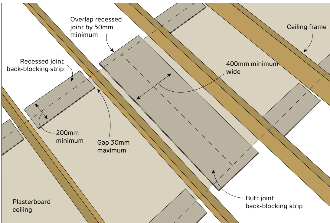
FIGURE 60 Placement of Back-Blocking Strips For Recessed and Butt Joints
