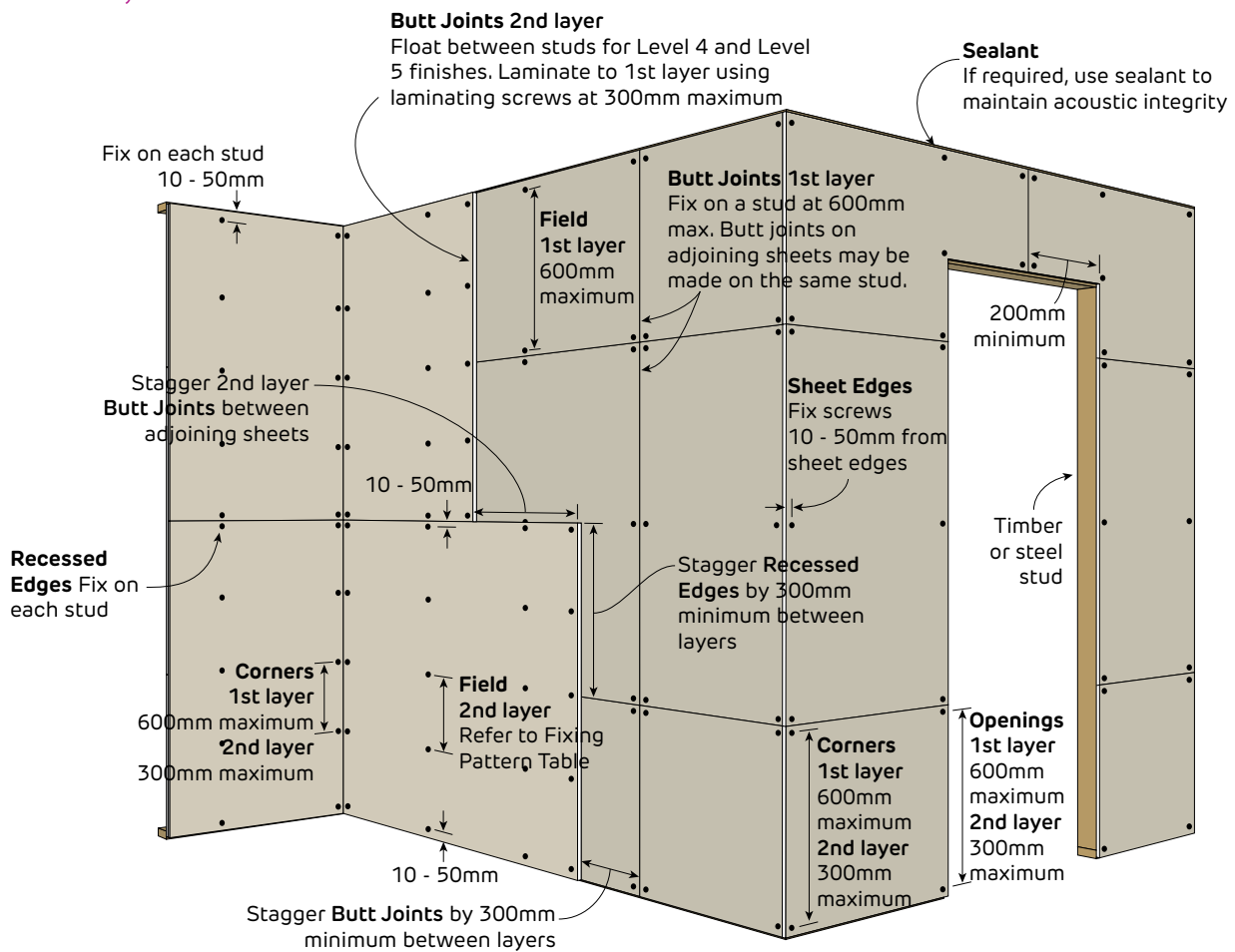
FIGURE 30 Internal Wall - 2 Layers Horizontal + Horizontal Fastener Only Method
