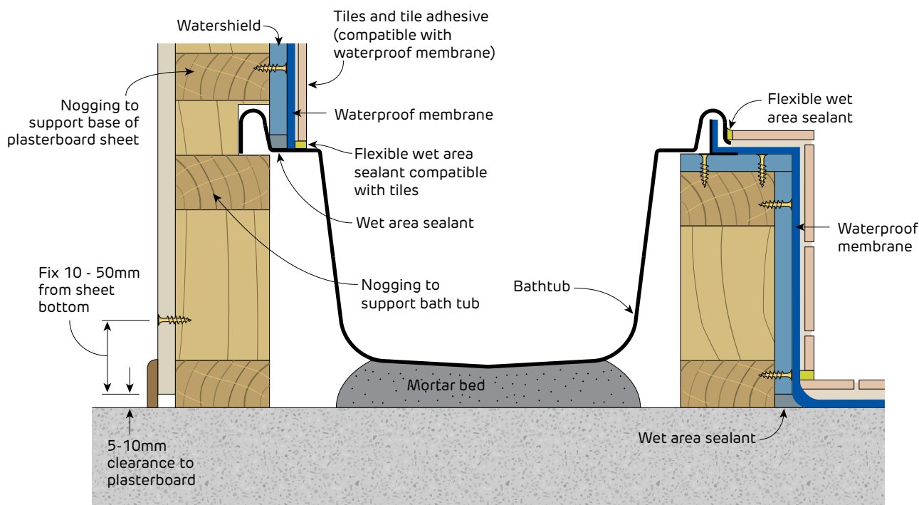
FIGURE 56 Bathtub Section
