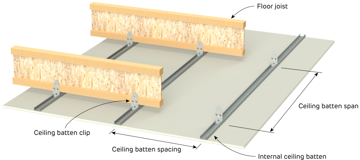
FIGURE 4 Internal Ceiling Batten Span and Spacing
