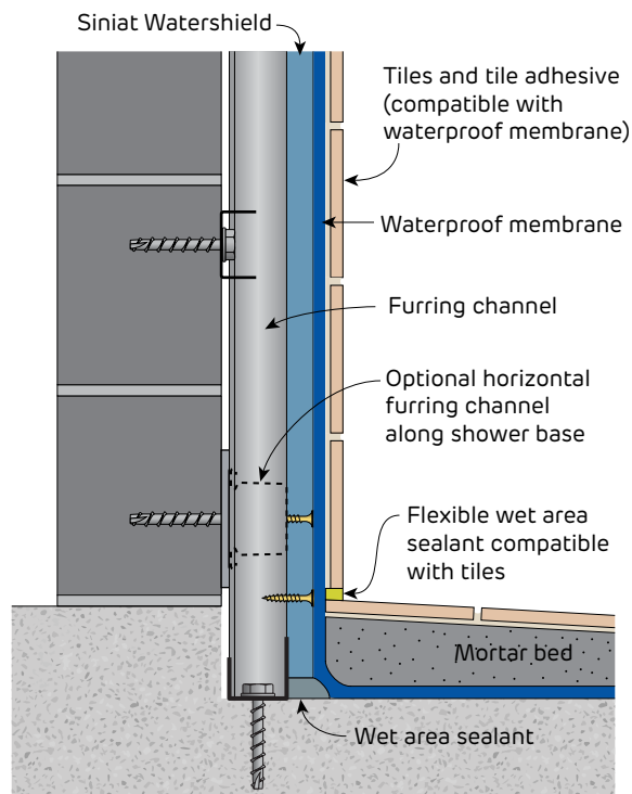
FIGURE 53 Shower Base over Masonry Wall Shower with dropdown Class 3 membrane shown - Section
