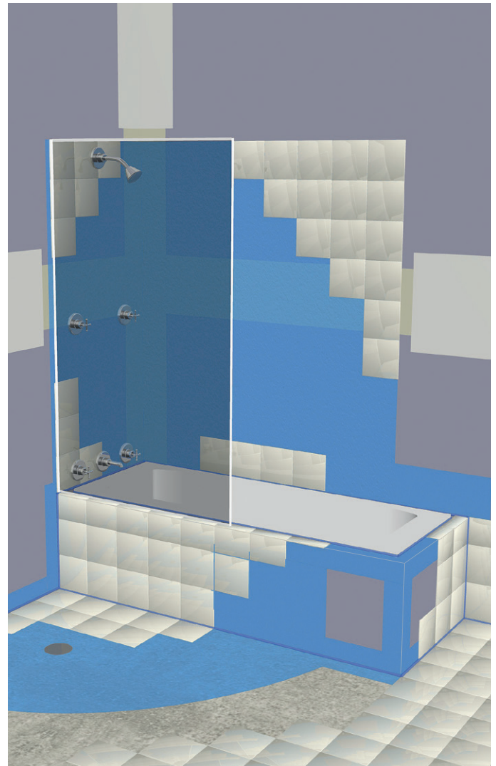
FIGURE 43 Bath with Shower over concrete floor
