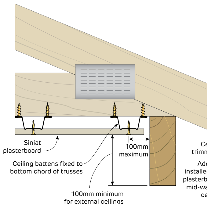
FIGURE 24 Plasterboard Ceiling Fixed to Battens Ceiling battens installed perpendicular to trusses Section
