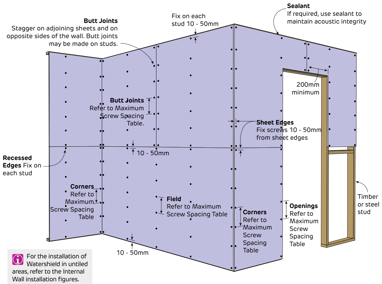
FIGURE 49 Watershield in Tiled Areas - 1 Layer Horizontal Screw Only Method
