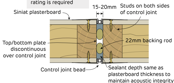
FIGURE 36 Wall Control Joint Plan
