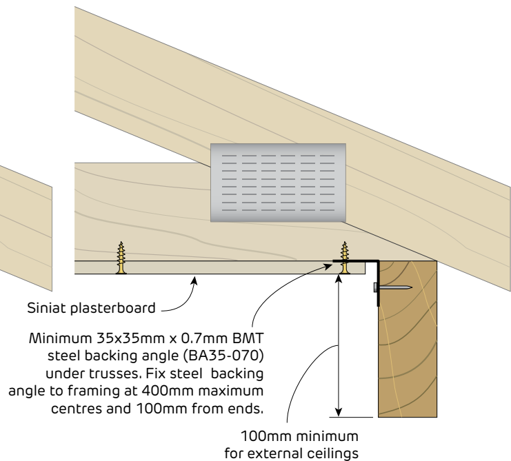
FIGURE 23 Plasterboard Ceiling Fixed to Roof Truss Alternative detail with perimeter steel angle Section
