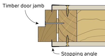
FIGURE 38 Timber Door jamb With Stopping Angle - Plan
