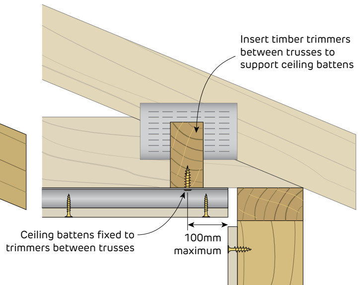
FIGURE 15 Direct Fix Ceiling to Roof Truss 22mm Cyclonic Batten parallel to trusses Section
