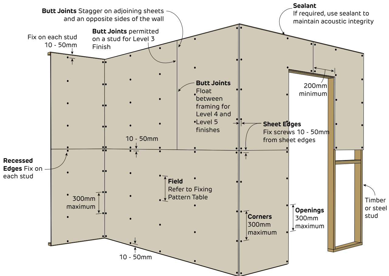
FIGURE 29 Internal Wall - 1 Layer Horizontal Fastener Only Method
