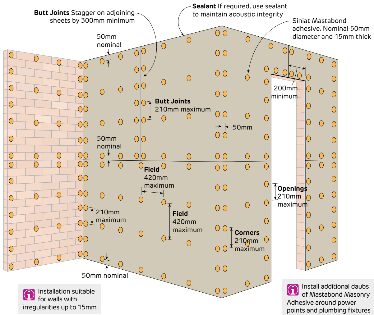
FIGURE 31 Internal Wall - 1 Layer Horizontal Masonry Adhesive Method
