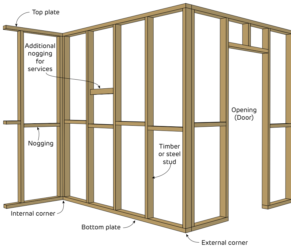
FIGURE 26 Wall Frame Layout
