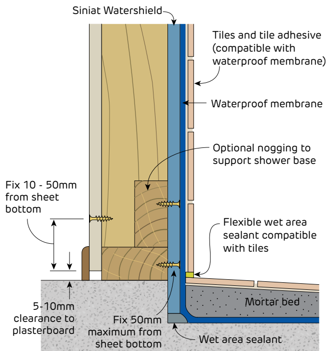
FIGURE 51 Shower Base Shower with dropdown Class 3 membrane shown - Section
